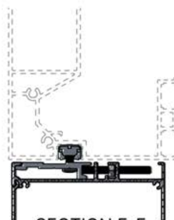
SECTION E-E
