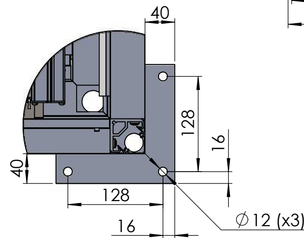
DETAIL C
